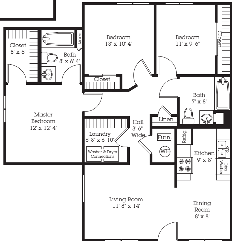
Lower Level
