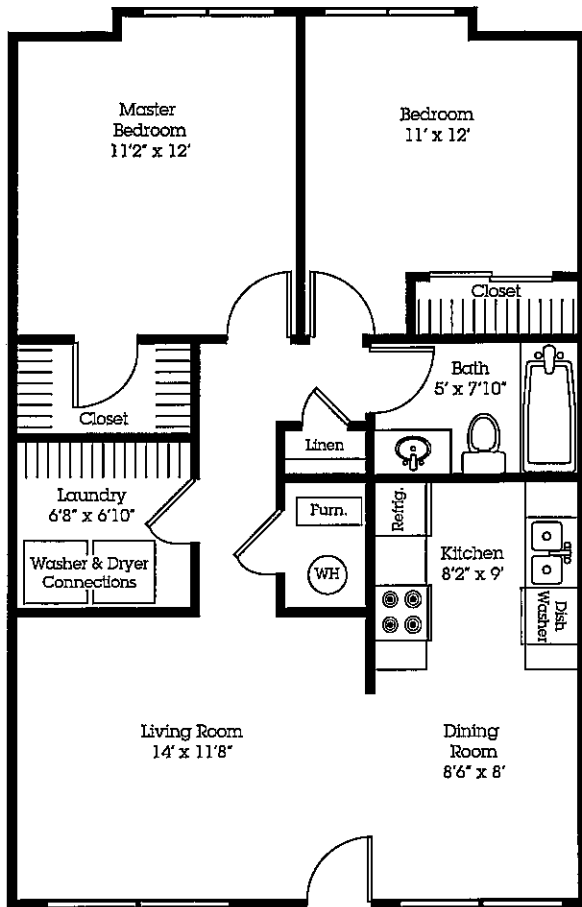
Upper Level
